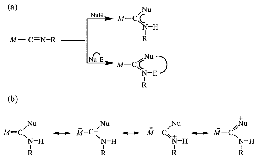
Scheme 1. (a) Activation of isocyanide toward nucleophilic addition ( \text{NuH} — protic nucleophile; \text{Nu} \text{---} \text{E} — nucleophile that also bears an electrophilic center) and (b) valence-bond representation of the derived aminocarbene ligand (exemplified for the case of the \text{NuH} nucleophiles).
