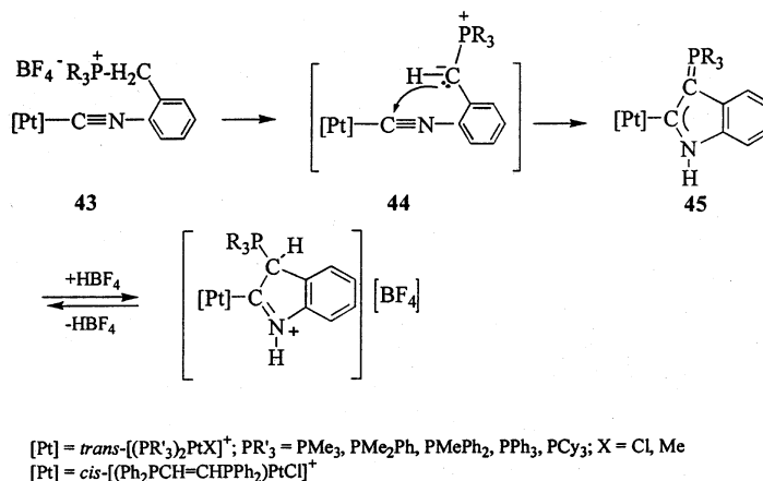
Scheme 9. Formation of cyclic aminocarbene Pt(II) complexes from cyclization of o -(phosphonomethyl)phenyl isocyanides [50,51].
