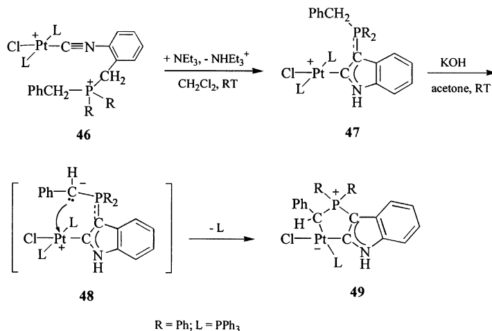
Scheme 10. Formation of aminocarbene platinaheterocycles from cyclization of benzylphosphonium-substituted isocyanides [52].
