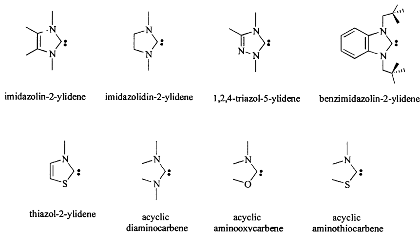
Scheme 19. Isolated cyclic and acyclic aminocarbenes [93].
